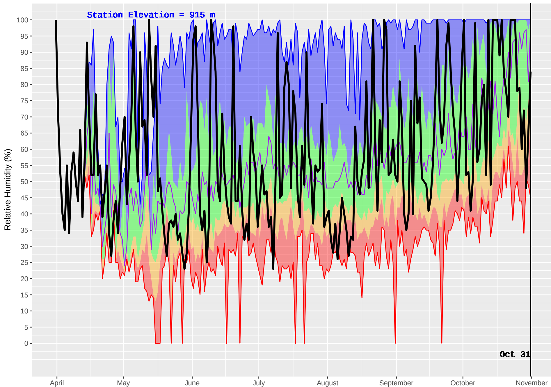
MCLEOD LAKE (153) : Historical (1990–2016) and Current (2017) Noon Relative Humidity
