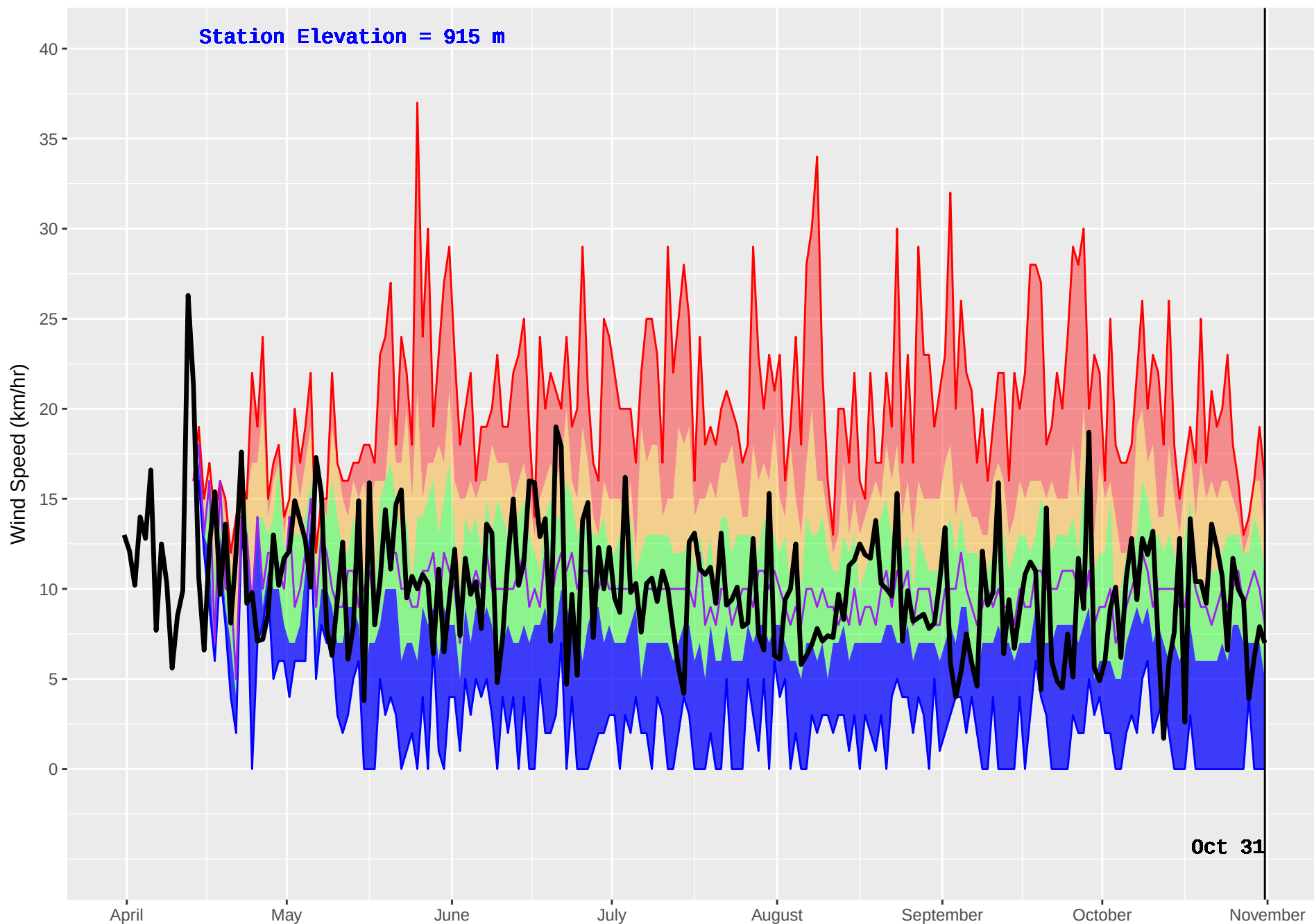
MCLEOD LAKE (153) : Historical (1990–2016) and Current (2017) Noon Wind Speed
