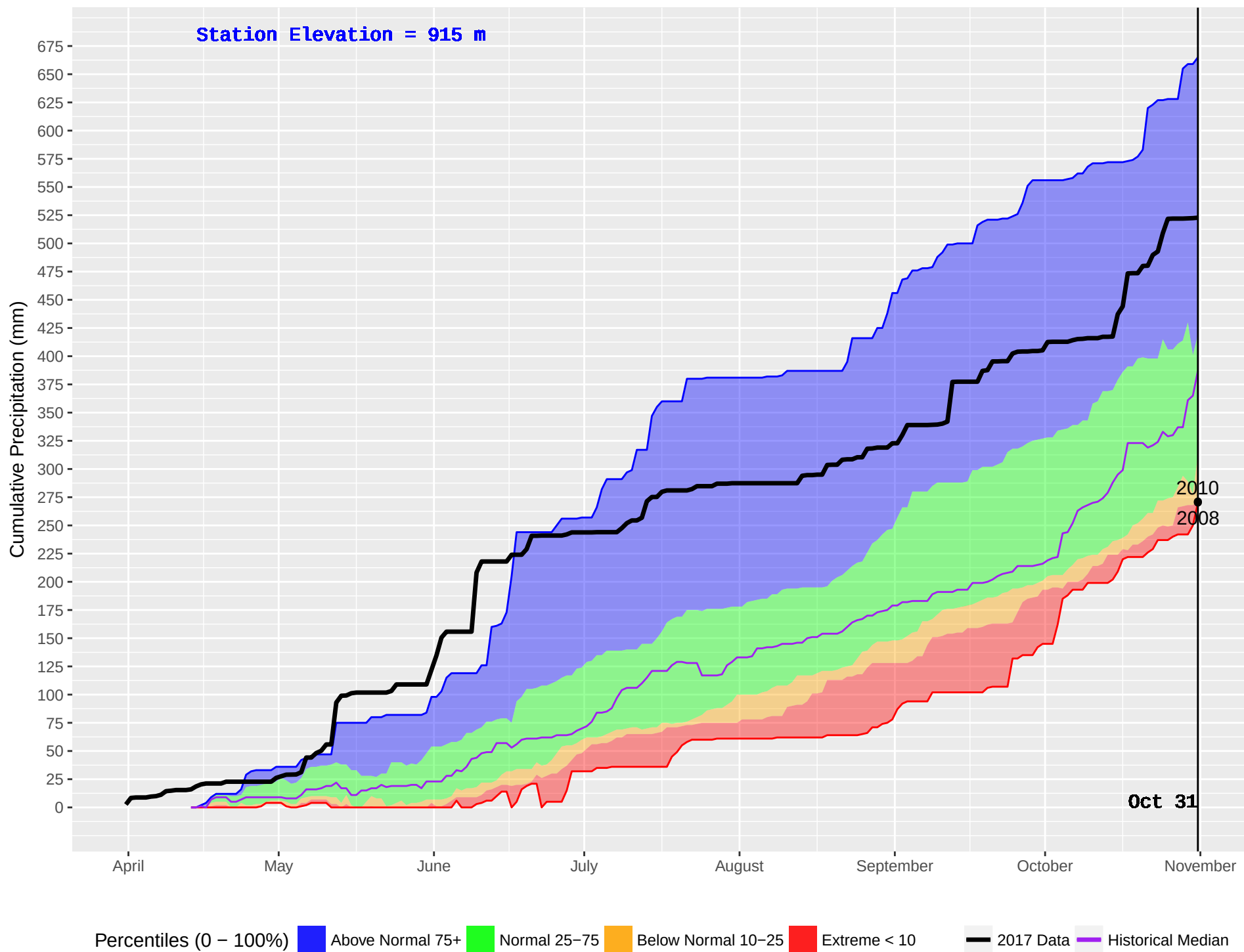
MCLEOD LAKE (153) : Historical (1990–2016) and Current (2017) Noon Cumulative Precipitation
