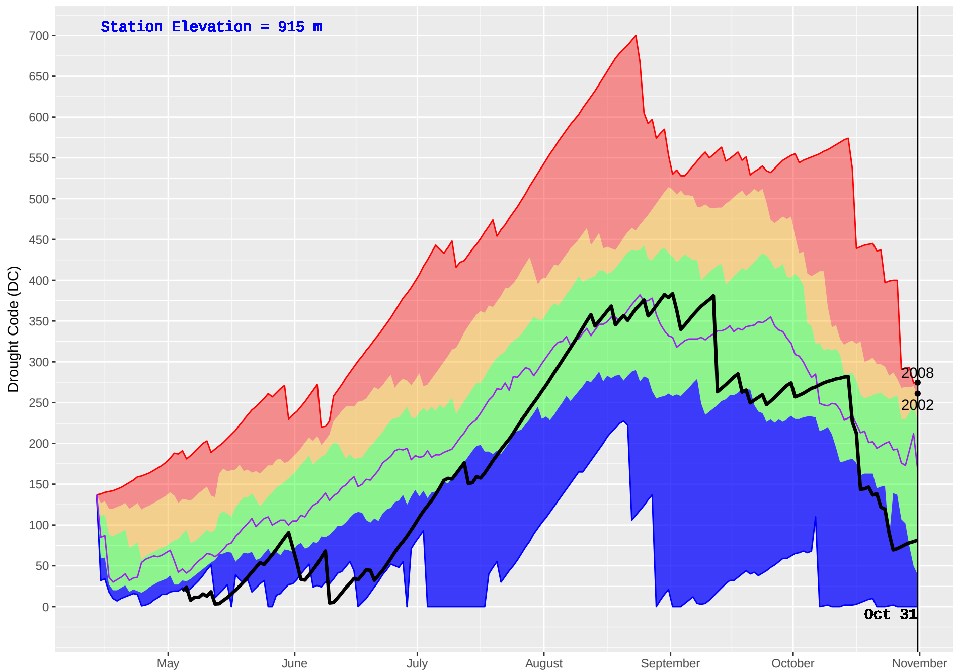
MCLEOD LAKE (153) : Historical (1990–2016) and Current (2017) Noon Drought Code (DC)
