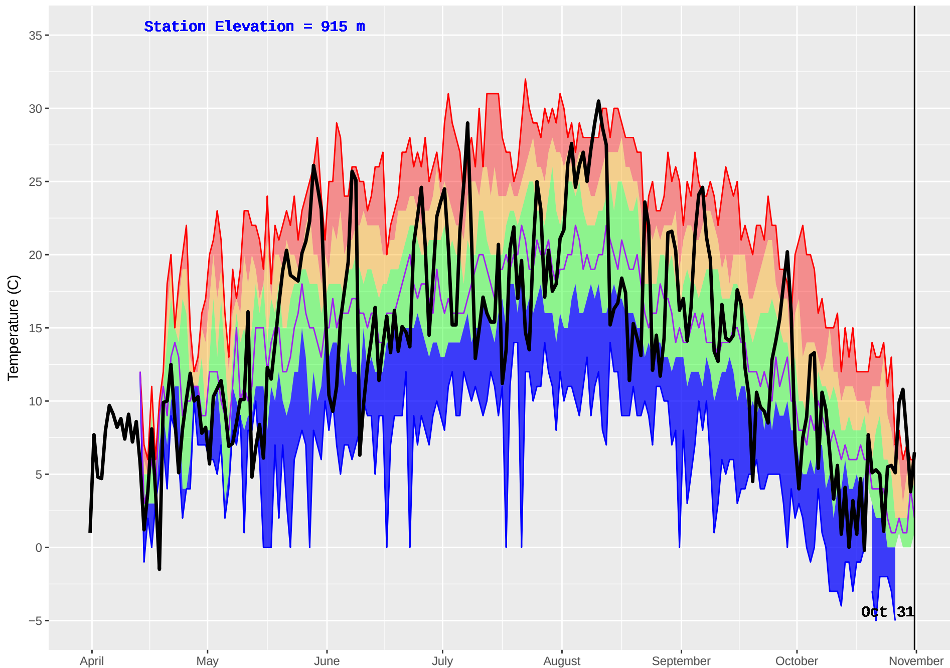
MCLEOD LAKE (153) : Historical (1990–2016) and Current (2017) Noon Temperature
